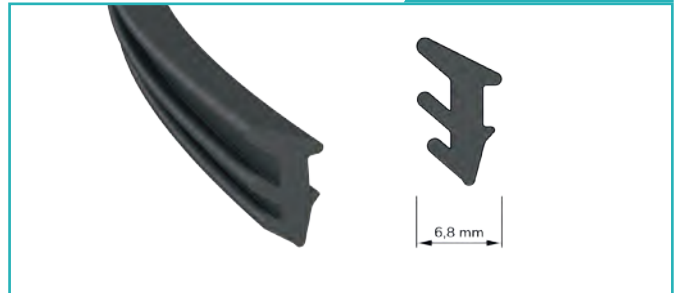
Tirnaklı Cam Contası Spiked Glass Joint
