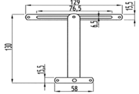
VASISTAS MAKAS VASISTAS OPENING MECHANISM
