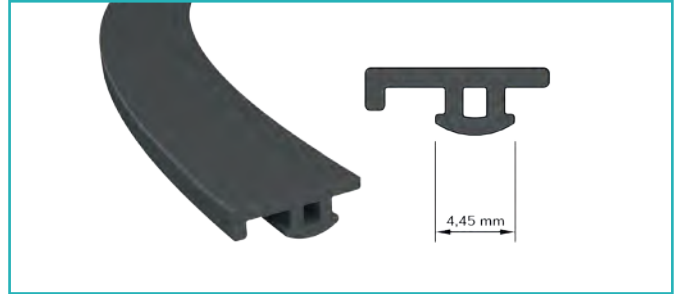
Çakma Conta Nailing Joint
