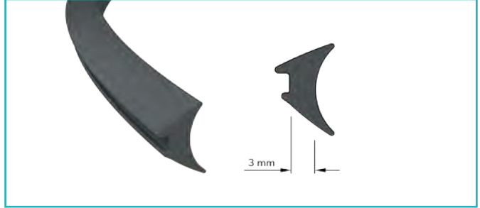
İç Cam Contası 3 mm. Interior Glass Joints 3 mm.
