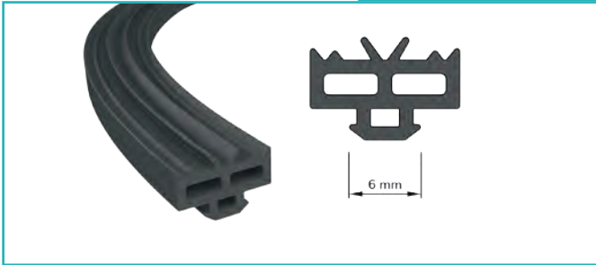
Cephe Cam Fitili Facade Glass Seal
