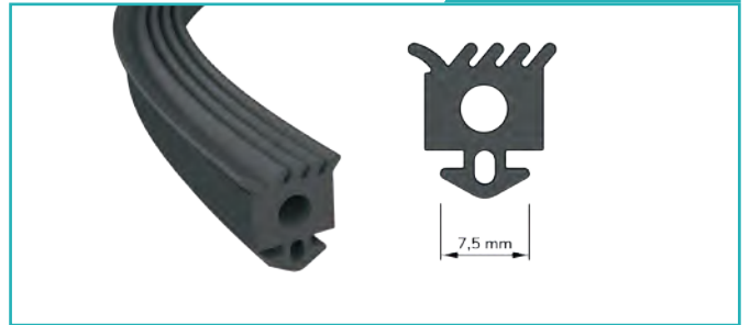
Mesafe Fiteli Distance Seal
