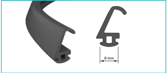
Toz Fitili Dust Seal
