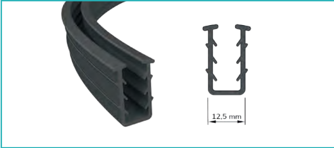
U Cam Fitili U Glass Seal
