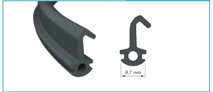
Tozluk Fitili Powder Seal
