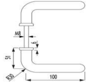
H KOL YAY MODEL PULL HANDLE
