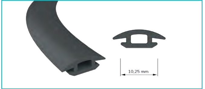
Ray Dolap Çarpma Fitili Seals For Sliding Folding Wardrobe
