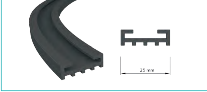
Kelepçe Fitili Clamp Seal
