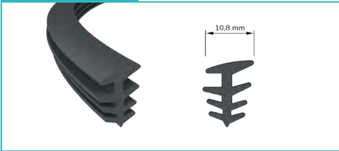
Tırnaklı Cam Fitili Spiked Glass Seal
