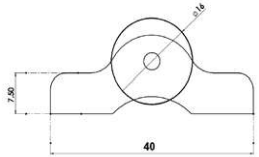
PİRİNÇ TEKLİ RULMAN ROLLER WITH ONE WHEEL BRASS ALLOY
