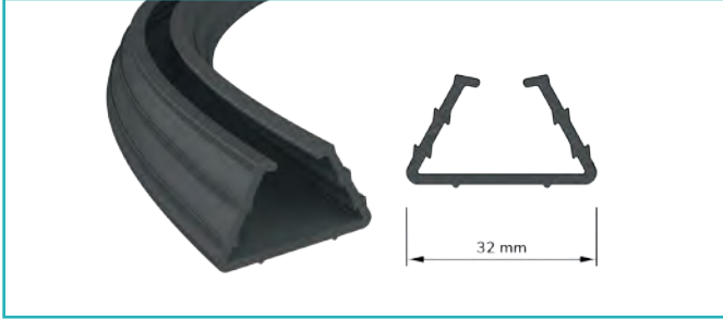
U Cam Fitiği U Glass Seal
