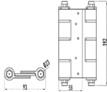
ÇARPMA KAPI MENTEŞESİ DESTEK SWINGING DOOR HANDLE COMPLEMENT
