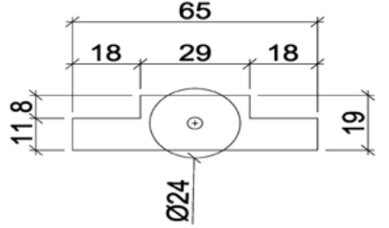
SİNEKLİK RULMAN ROLLER SWATTER
