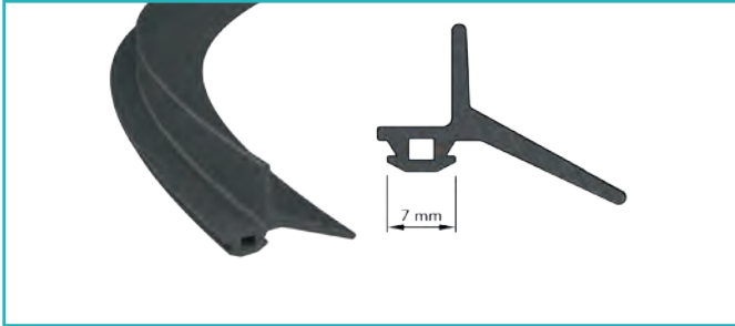
Tozluk Fiteli Powder Seal
