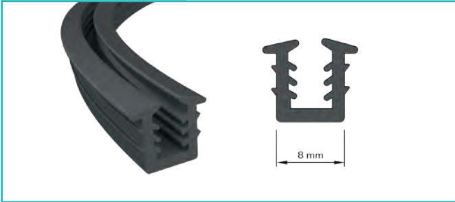
Cam Fiteli Glass Seal
