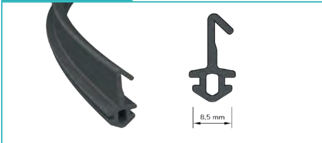
Tozluk Cam Fitili Powder Glass Seal
