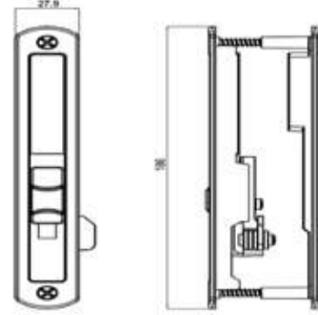
SÜRME KİLİT GAGALI RECESSED SLIDING HANDLE
