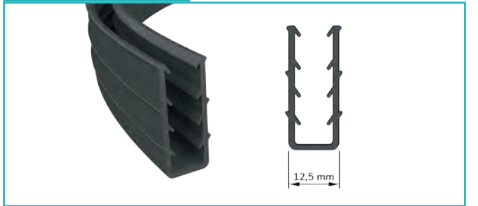
U Cam Fitili U Glass Seal
