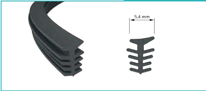
Tirnaklı Cam Fitili Spiked Glass Seal
