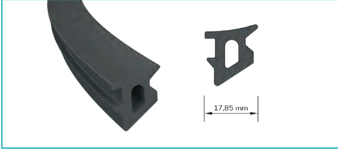
İç Cam Contası 17,85 mm. Interior Glass Joints 17,85 mm.
