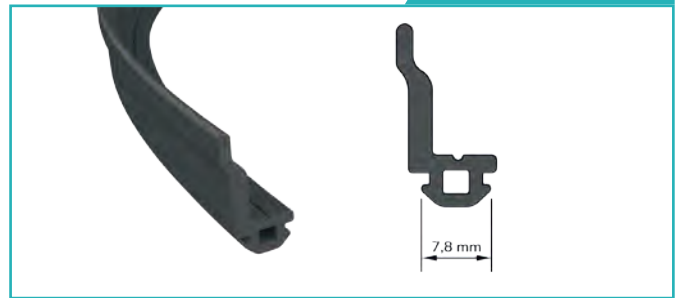
Tozlu Fıtlı Powder Seal
