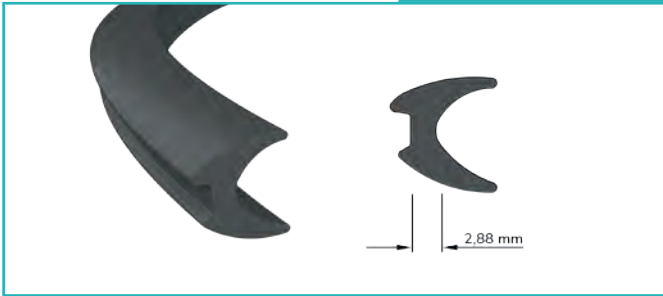
Genel Fitil General Seal
