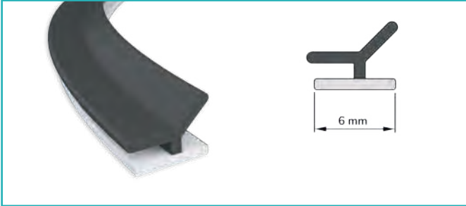
Sert Yumuşak Aldoks Çift kulak 6 mm. Hard Soft Aldoks Double Ear 6 mm.
