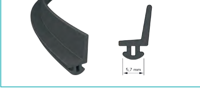
Tozluk Fitili Powder Seal
