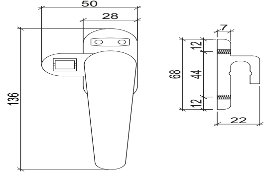
MAFSALLI CEPHE KOL FACADE WINDOW HANDLE
