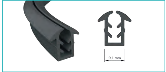
U Cam Fiti U Glass Seal
