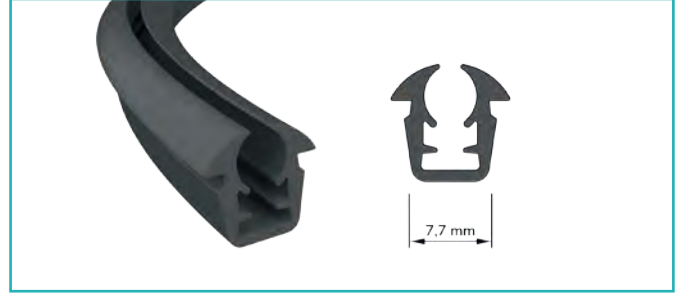
Cam Fiti Glass Seal
