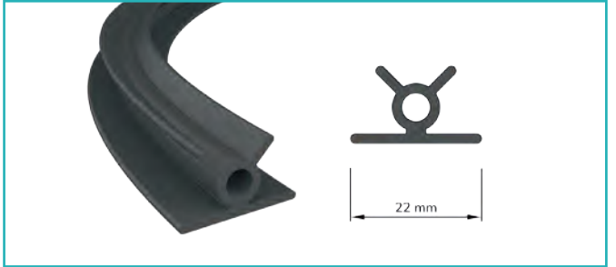
Genel Fitil General Seal
