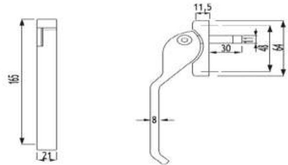
GIZLI KANAT KOL CREMONE HANDLE (OUTWARD OPENING)
