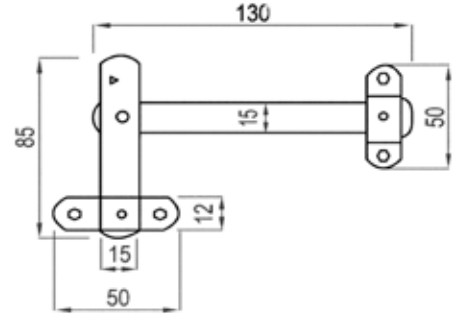
3 KADEMELİ MAKAS VASISTAS OPENING MECHANISM
