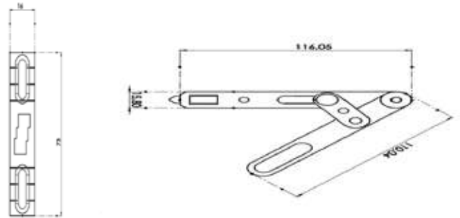
VASISTAS MAKAS VASISTAS OPENING MECHANISM
