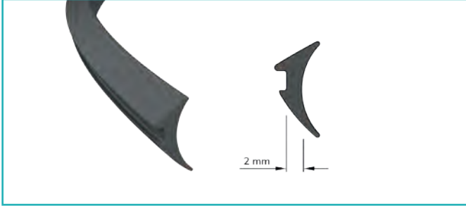
İç Cam Contası 2 mm. Interior Glass Joints 2 mm.
