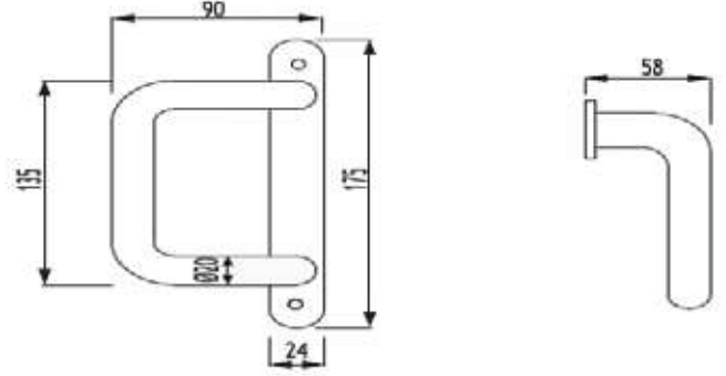
MINİ U KOL TAKIM PULL HANDLE
