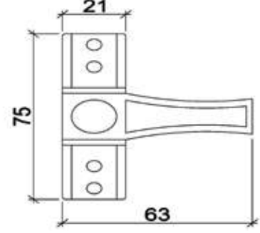
YAYLI EMNİYET KİLİDİ 3 WINDOW SAFETY LOCK 3
