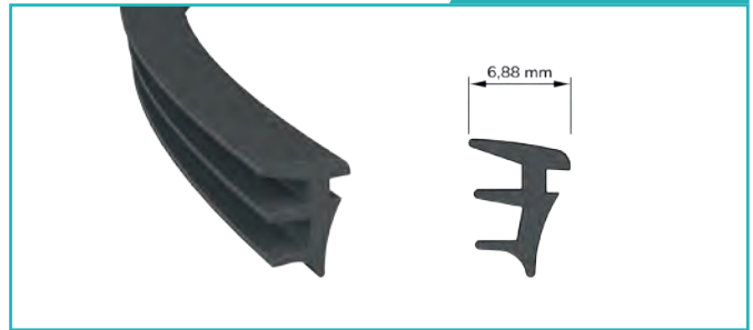
Cam Fitili Glass Seal
