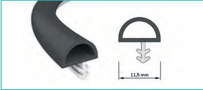
Sert Yumuşak Ahşap Doğrama Fitili Hard Soft Wood Work Seal
