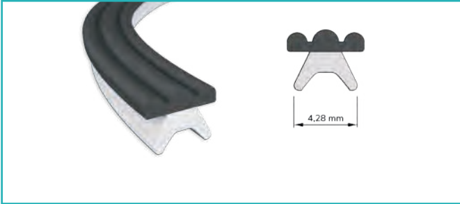
Sert Yumuşak Panjur Hard Soft Louver
