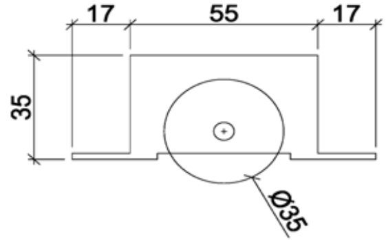
ÇİFT TEKER PİRİNÇ RULMAN ROLLER WITH DOUBLE WHEEL BRASS ALLOY
